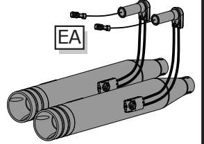
Exhaust/cable/ servo system
